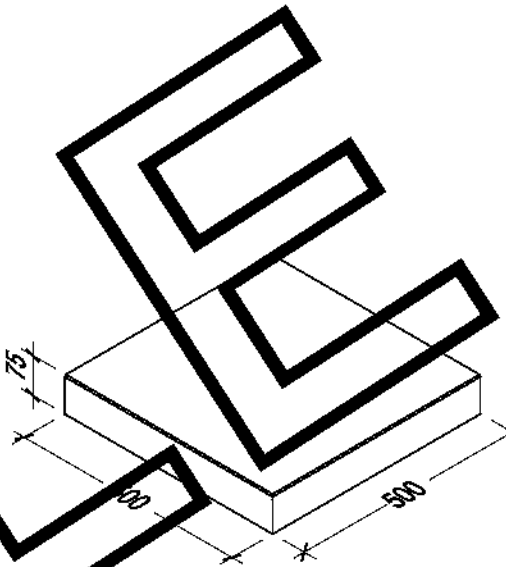
PRE-CAST PAVING BLOCK TYPE "C" NOT TO SCALE
